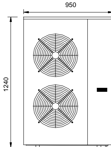
Dimensions (MM)
