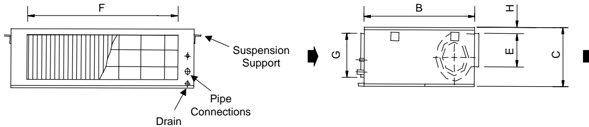
Dimensions (MM)
