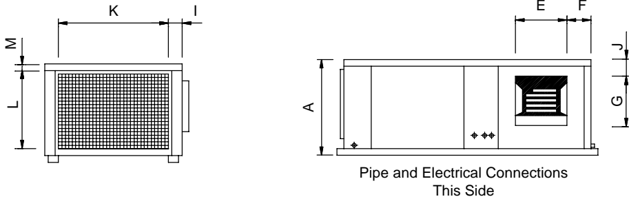
Dimensions (MM)
